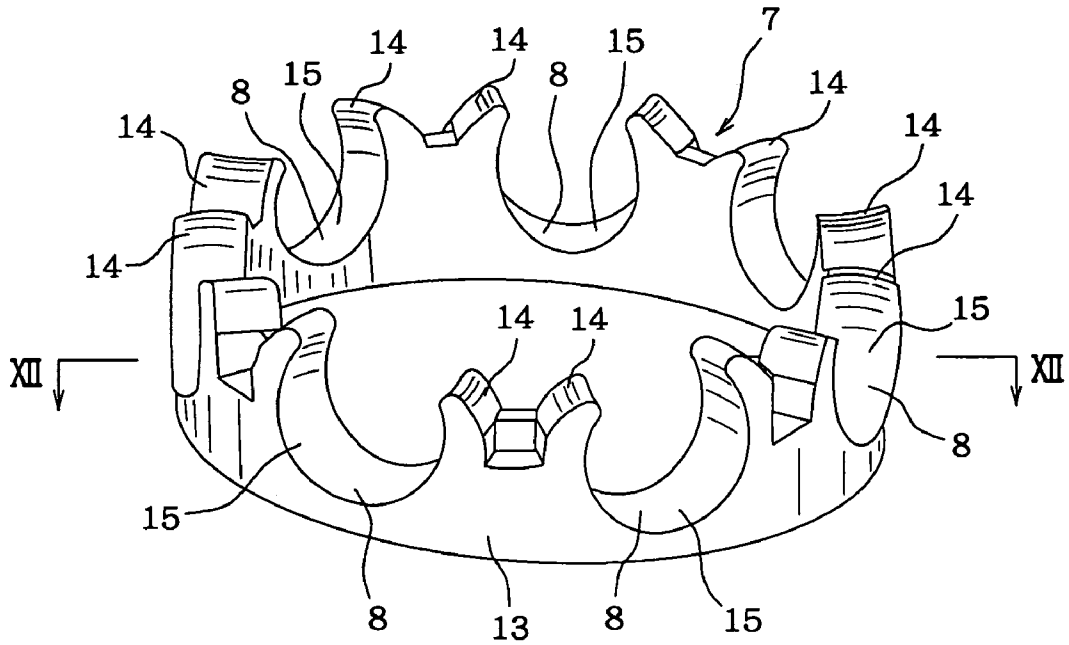
Fig. 2 PRIOR ART
